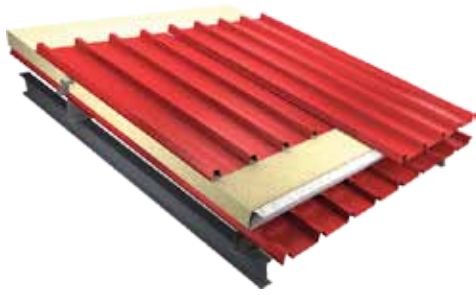
ROOF PROFILING
