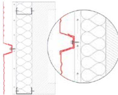
FACADE PROFILING HORIZONTAL INSTALLATION CROSS SECTION
