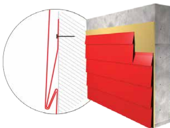
HORIZONTAL INSTALLATION
