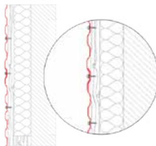
FACADE PROFILING HORIZONTAL INSTALLATION CROSS SECTION
