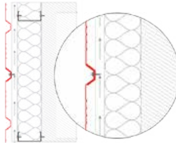
FACADE PROFILING HORIZONTAL INSTALLATION CROSS SECTION
