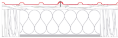
ROOF PROFILING INSTALLATION CROSS SECTION
