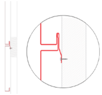
INSTALLATION DETAIL
