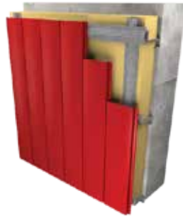
VERTICAL INSTALLATION
