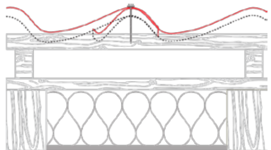
INSTALLATION DETAIL
