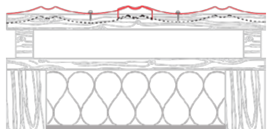
INSTALLATION DETAIL
